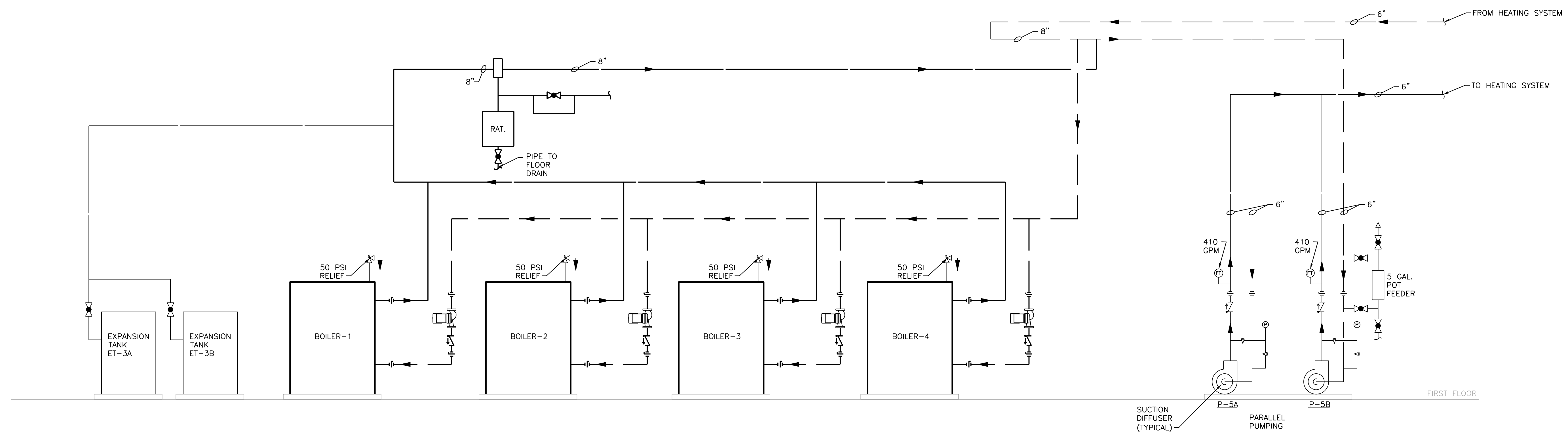
HEATING WATER SCHEMATIC - REVISED SCALE: NONE
