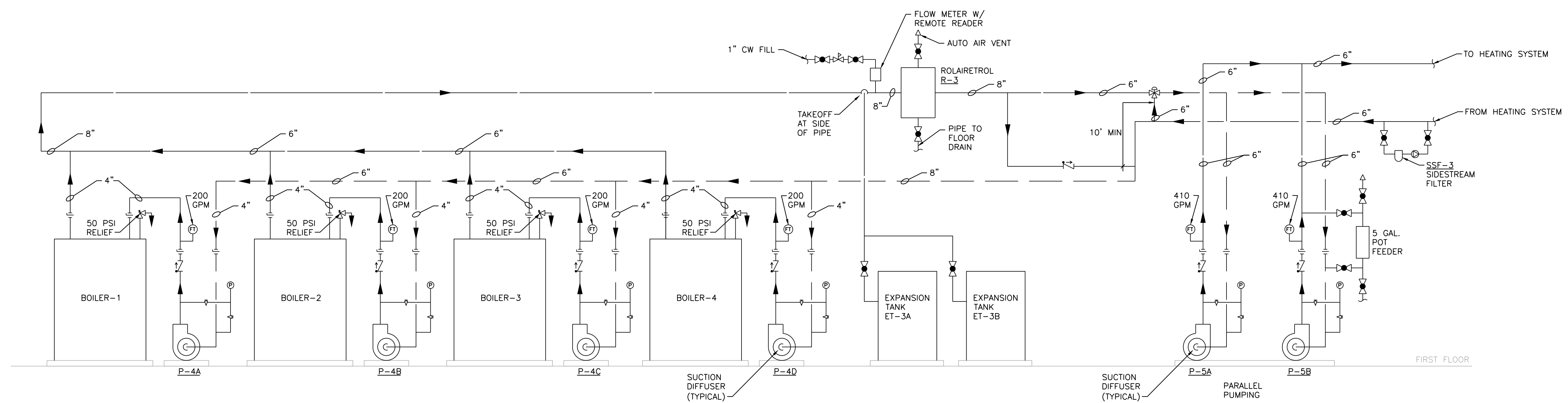
HEATING WATER SCHEMATIC - EXISTING SCALE: NONE
